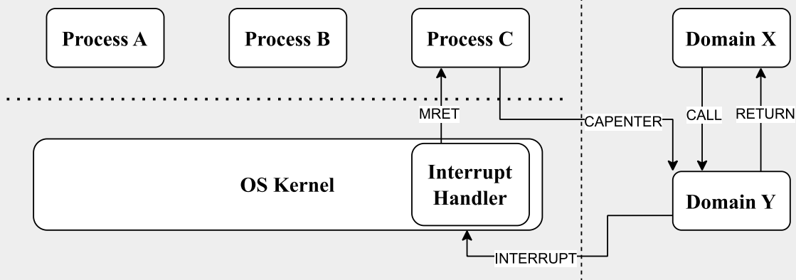
Figure 54. Overview of interrupt handling in TransCapstone
