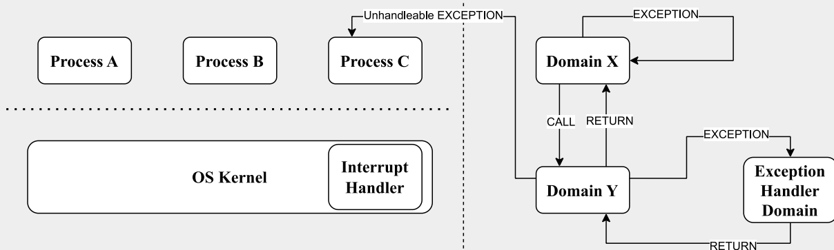
Figure 54. Overview of exception handling in TransCapstone
