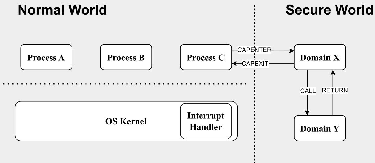
Figure 28. Overview of world switching in TransCapstone
