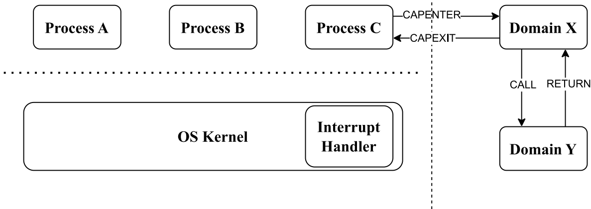
Figure 28. Overview of world switching in Capstone-RISC-V
